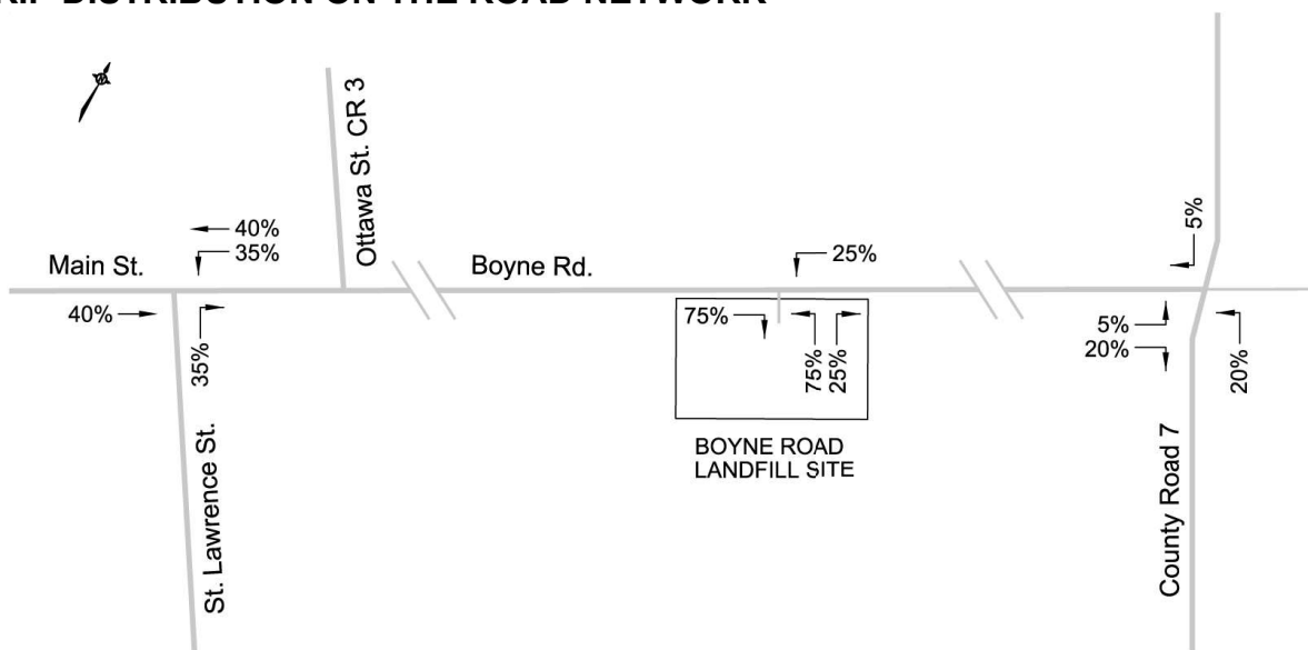
FIGURE 5.1 TRIP DISTRIBUTION ON THE ROAD NETWORK
