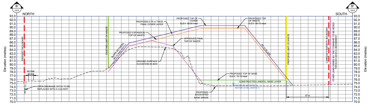
HORIZ. SCALE 1:1,500 m (B-B) SECTION VERT. SCALE 1:300 m (B-B) SECTION
