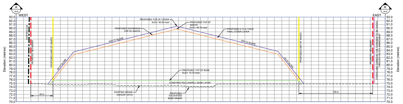
HORIZ. SCALE 1:1,500 m A-A' SECTION VERT. SCALE 1:300 m 10-5
