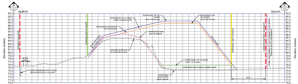
HORIZ. SCALE 1:1,500 m B-B' SECTION VERT. SCALE 1:300 m 10-5
